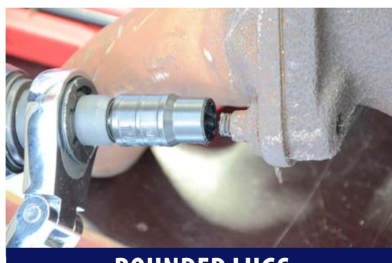
ROUNDED LUGS For this use twist sockets
